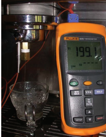
Figure 3. Installed portafilter thermometer measuring the temperature of the metered brew water stream.
